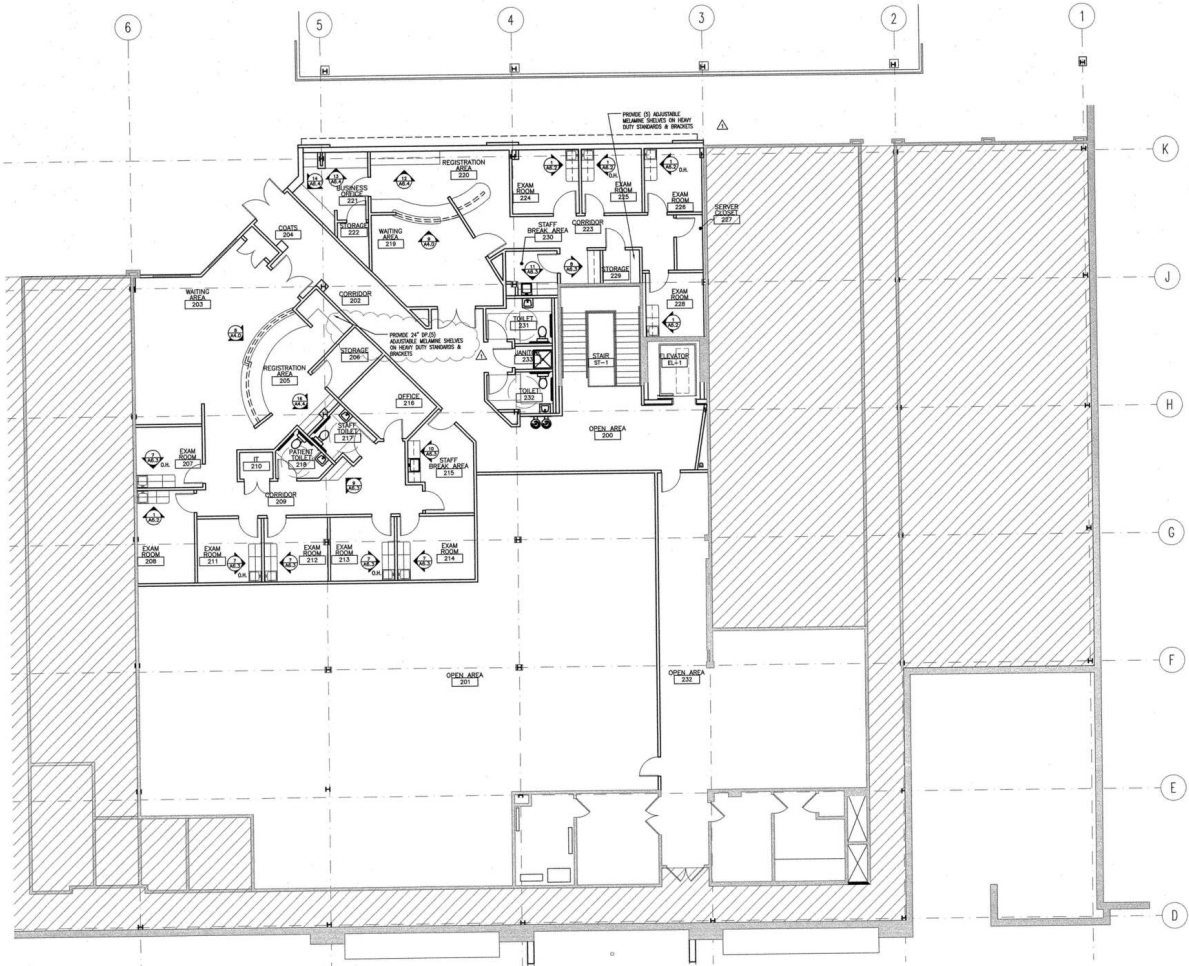
SECOND FLOOR MILLWORK PLAN SCALE: 1/8"=1'-0"
