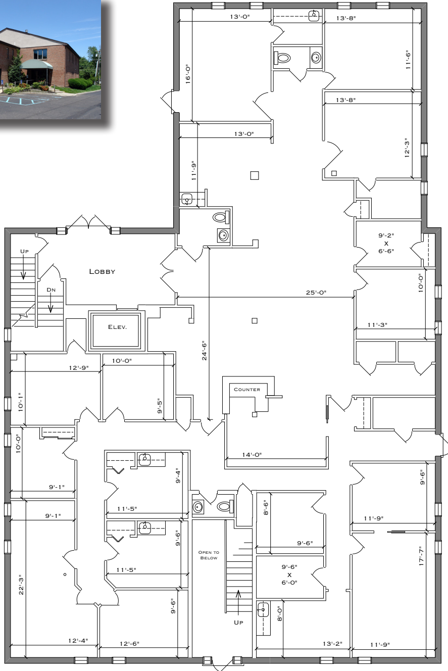
1st Floor - 4,980 SF
