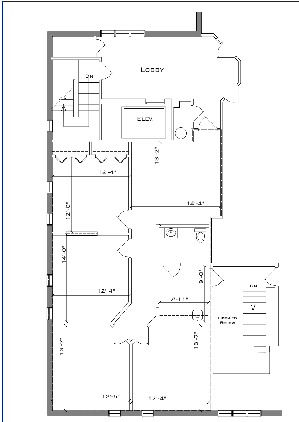
2nd Floor - 1,300 SF
